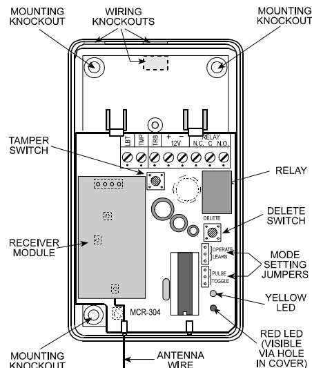
Figure 2. MCR-304 with Cover Removed
